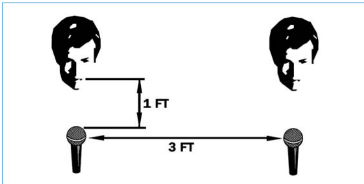
Figure 8: 3-to-1 rule
