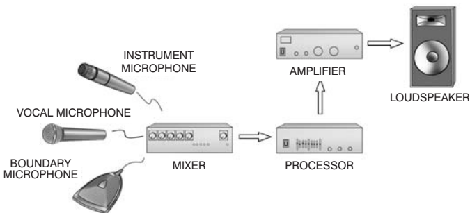
Figure 15: Typical sound system
