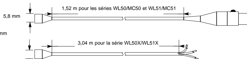
DIMENSIONS MICROPHONE ET CÂBLE FIGURE 3
