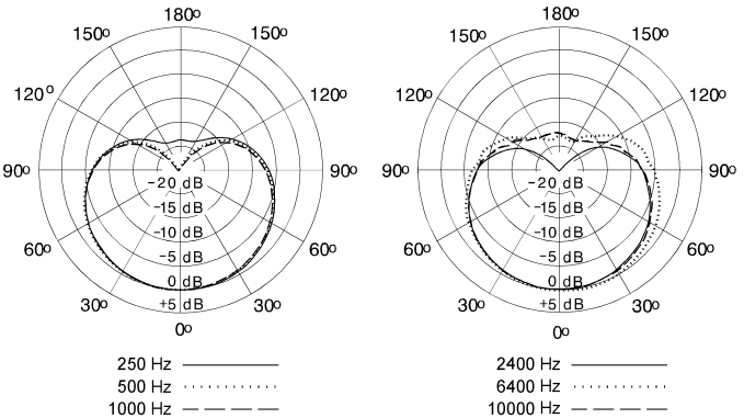
FIGURE 2. COURBES DE DIRECTIVITE TYPQUES
