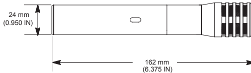
FIGURE 3. DIMENSIONS
